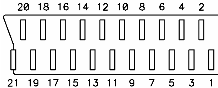
SCART female connector, front view.
